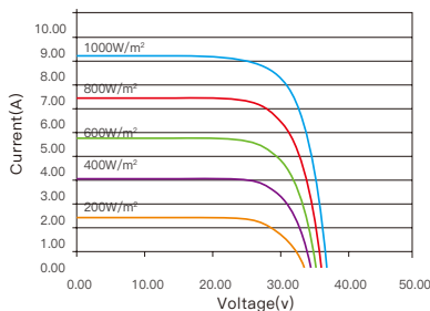
IV CURVE
