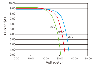
IV CURVE
